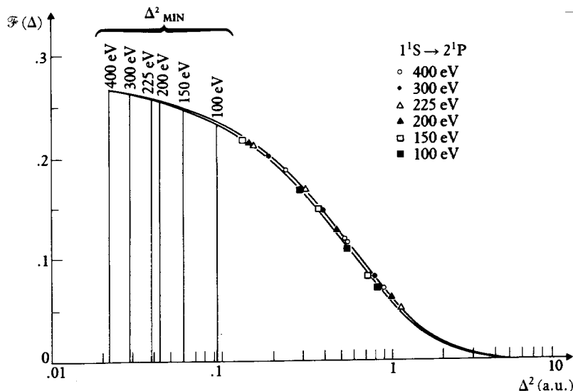
12.6 Generalised oscillator strength in atomic units for excitation of helium to the 2^1P level from the ground state.
